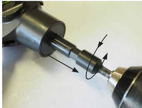
Fig. 2.1 If cutters are pre-installed, use your drill to ensure that both the hex drive and cutter end of the cutter assembly are fully retracted.
