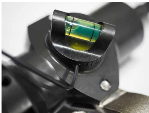
Fig. 4.1 Loosen the two grub screws with the Allen key to adjust the angle setter.
